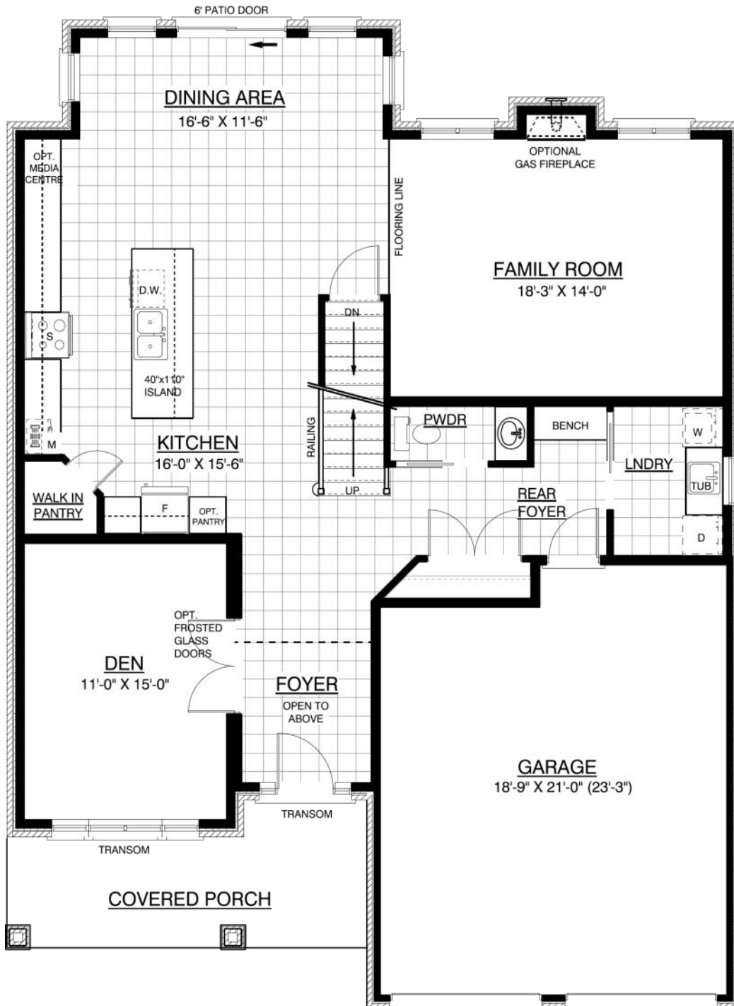
Main Floor Plan - 1,356 sqft
