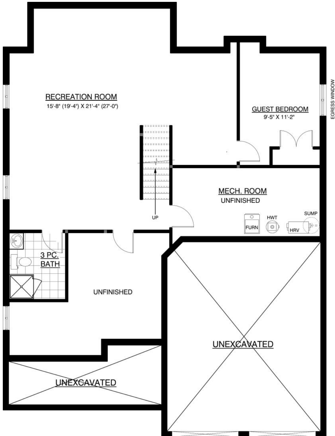
Optional Finished Basement Plan - 840 sqft finished area
