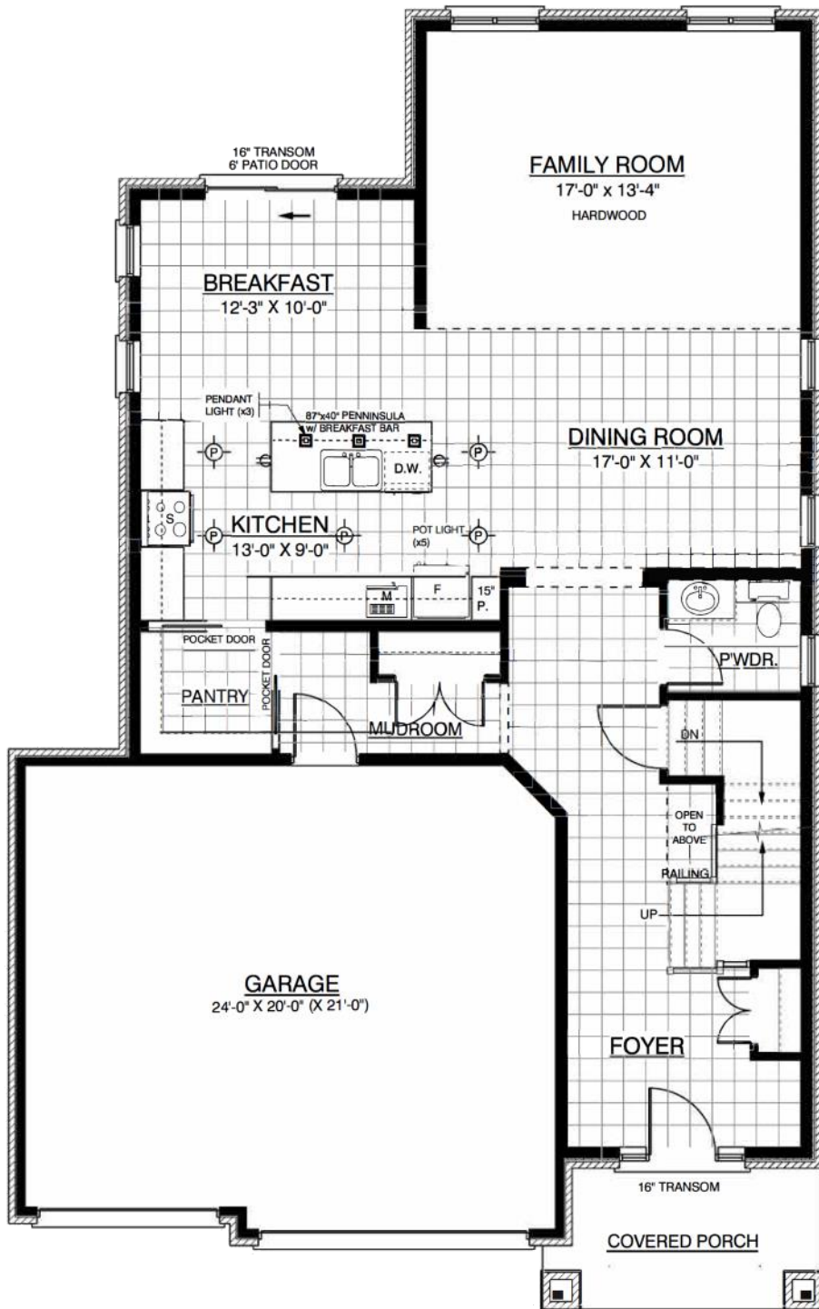
Main Floor Plan - 1,208 sqft
