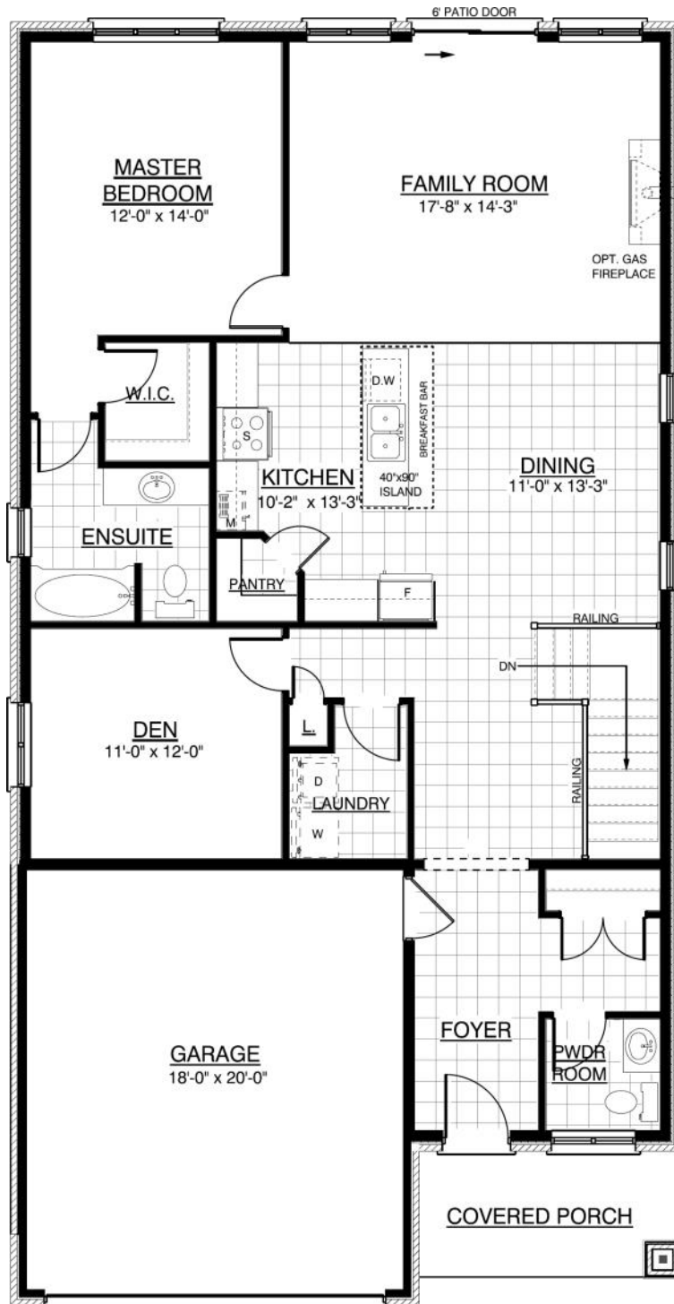
Main Floor Plan "B" - 1 Bedroom & Den - 1,458 sqft
