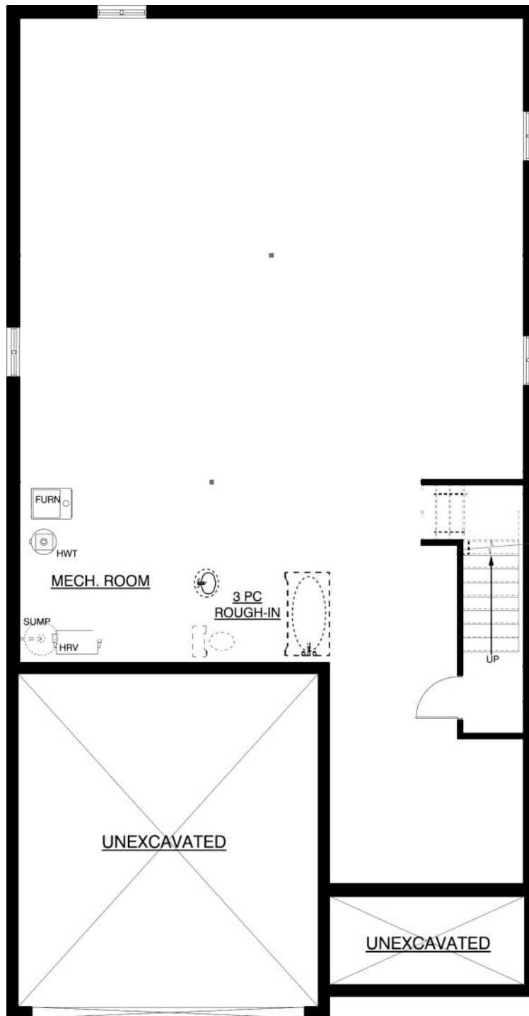
Standard Unfinished Basement
