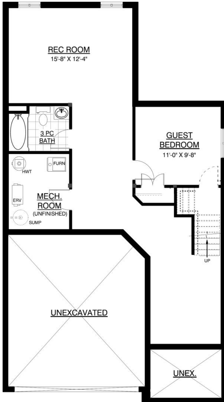
Optional Finished Basement - 730 sqft finished area
