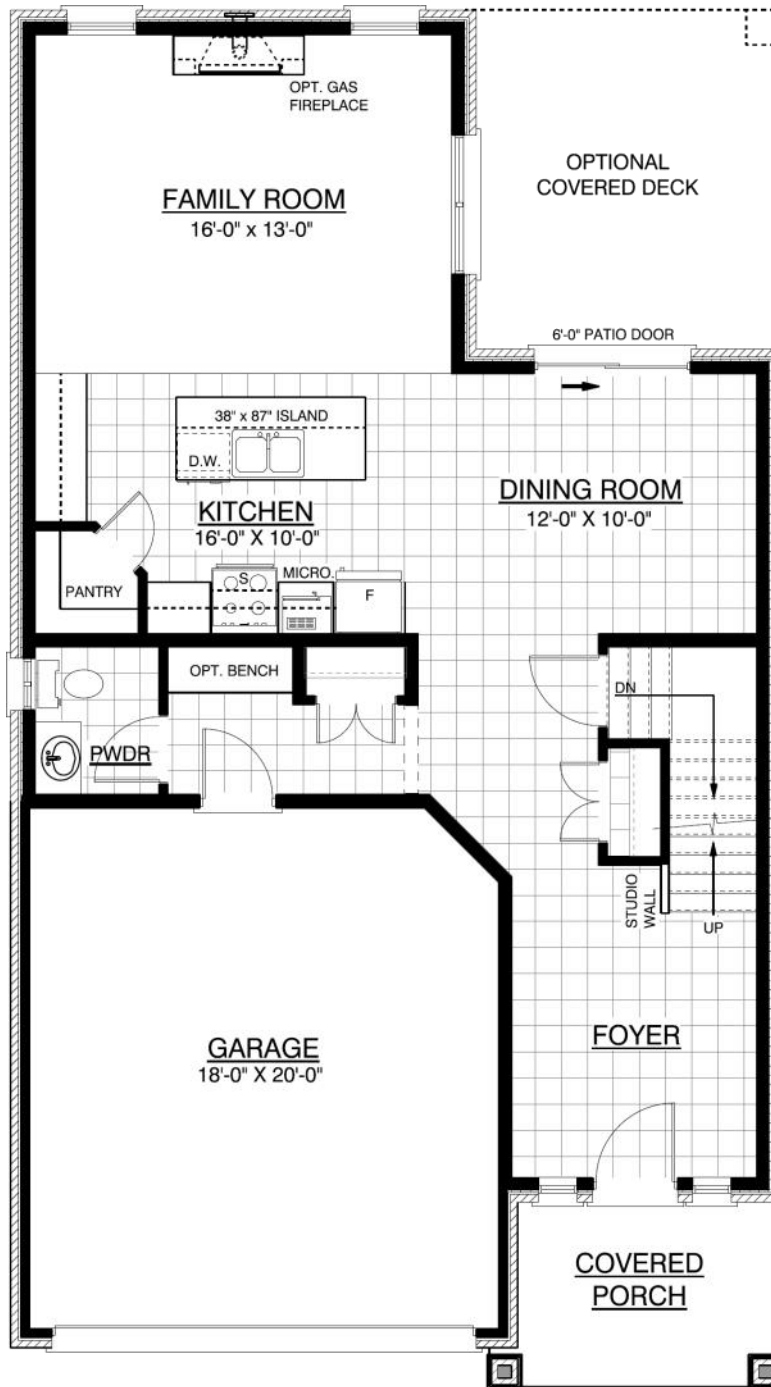
Main Floor Plan - 918 sqft
