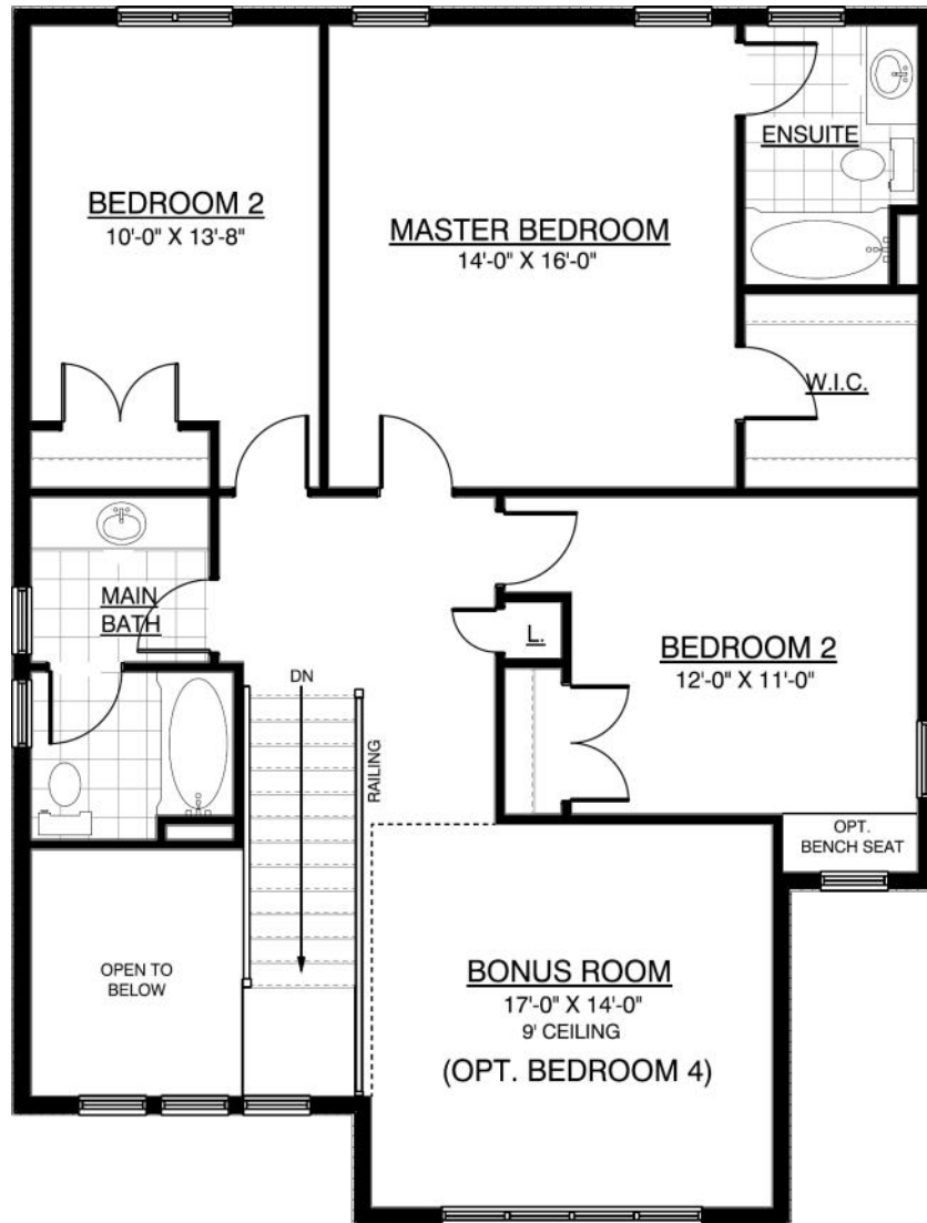
Upper Floor Plan - 1,126 sqft
