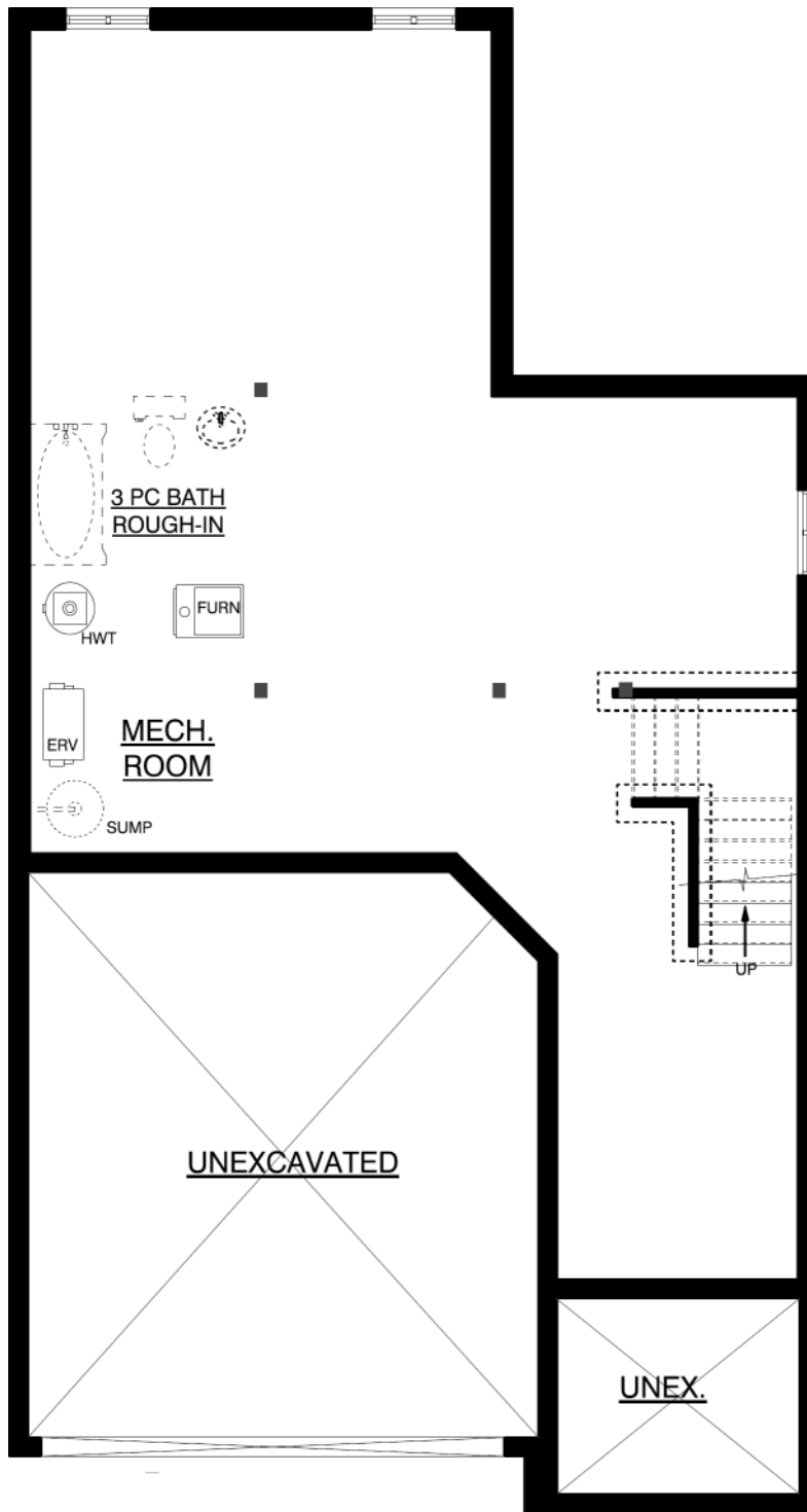
Basement Plan
